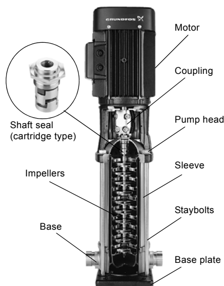
Fig. 3 CR pump
