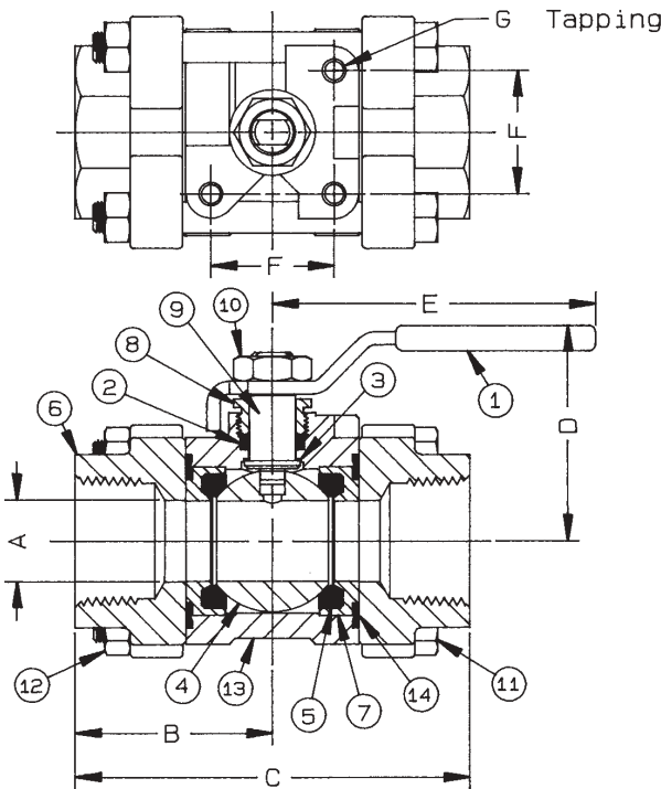
STAINLESS STEEL 3-PIECE HIGH PRESSURE FULL PORT BALL VALVE
